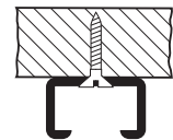
CEILING MOUNT COUNTER SINK SCREW
