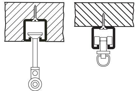
RECESSED MOUNT CEILING MOUNT
