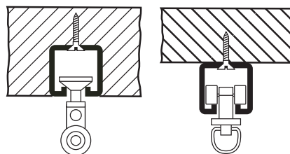
RECESSED MOUNT CEILING MOUNT
